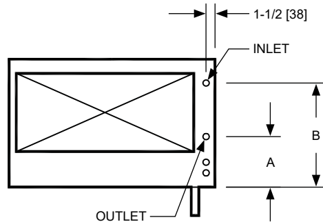
TOP VIEW (FILTER RACK OMITTED) (RIGHT HAND UNIT)
